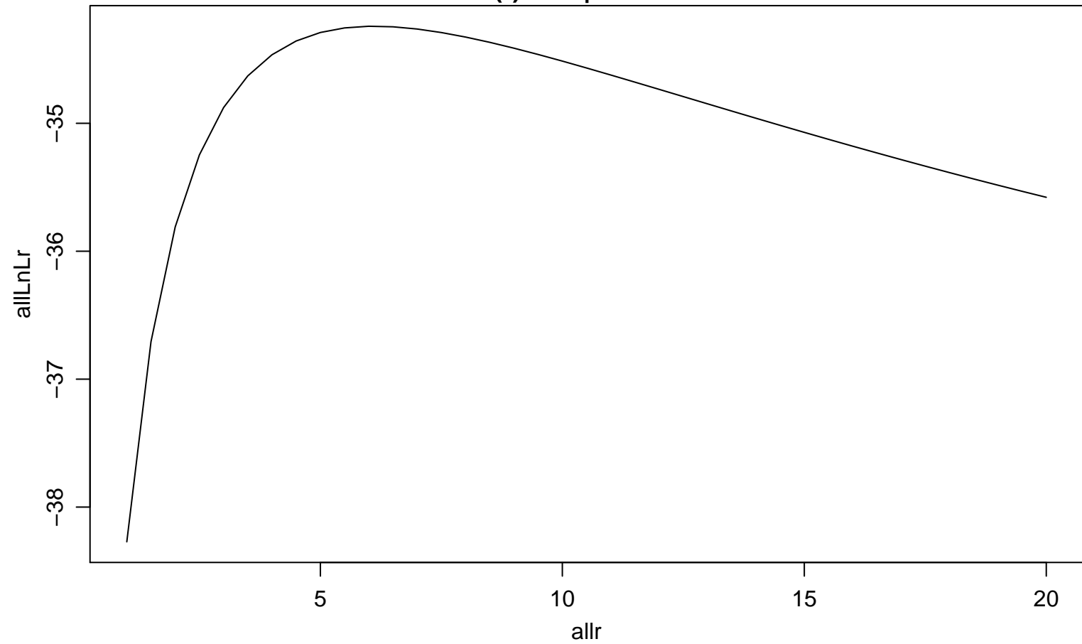
\ln L(r) vs r | \mu = 16.4
