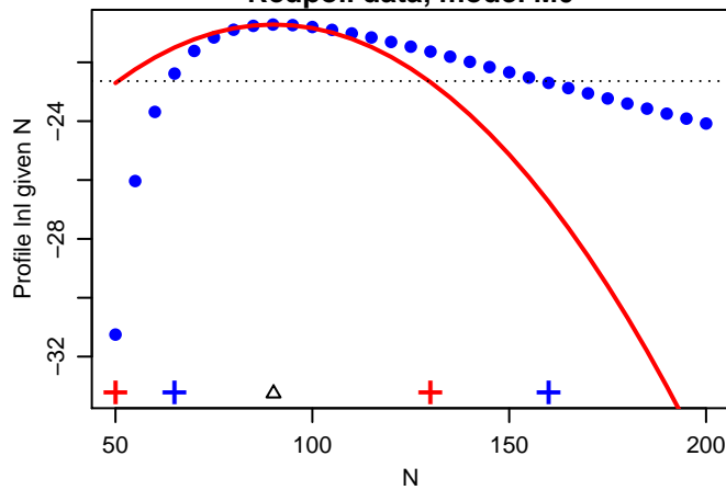
2 x Redpoll data, model M0
