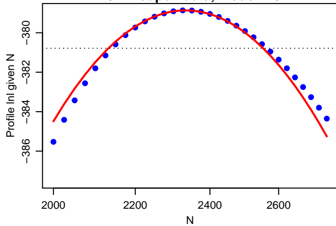
25 x Redpoll data, model M0
